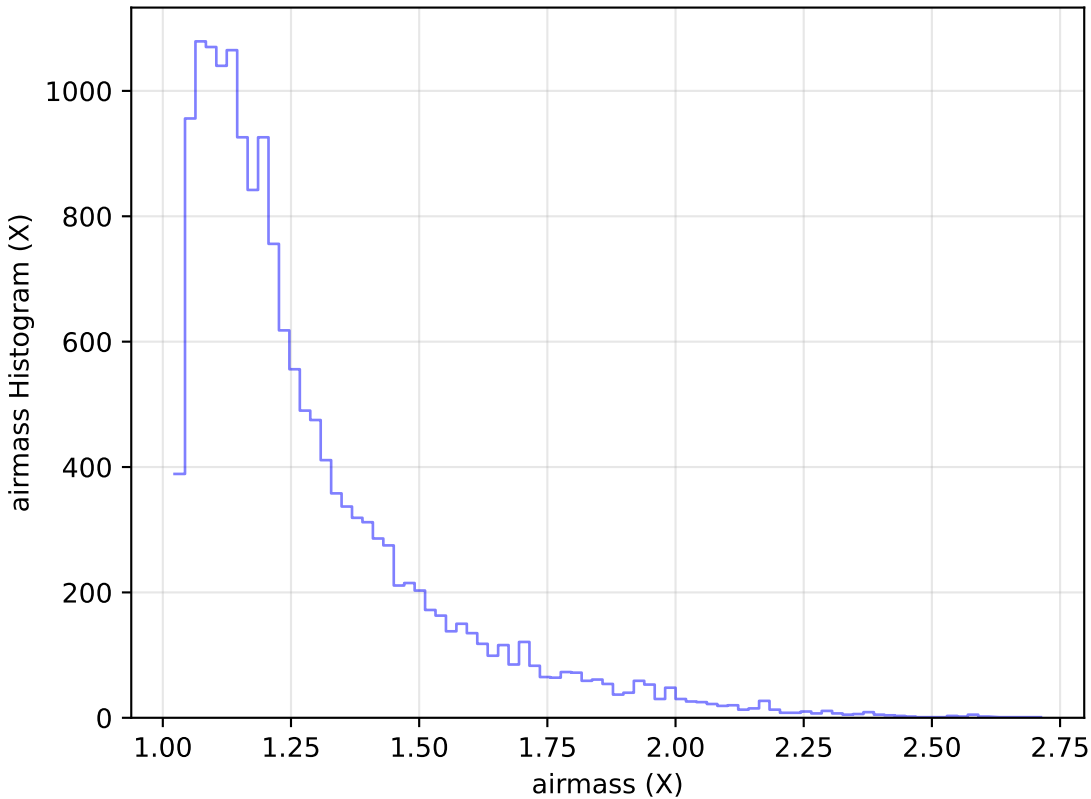
too_100_1v3.4_10yrs Yr 1 u band: airmass Histogram
