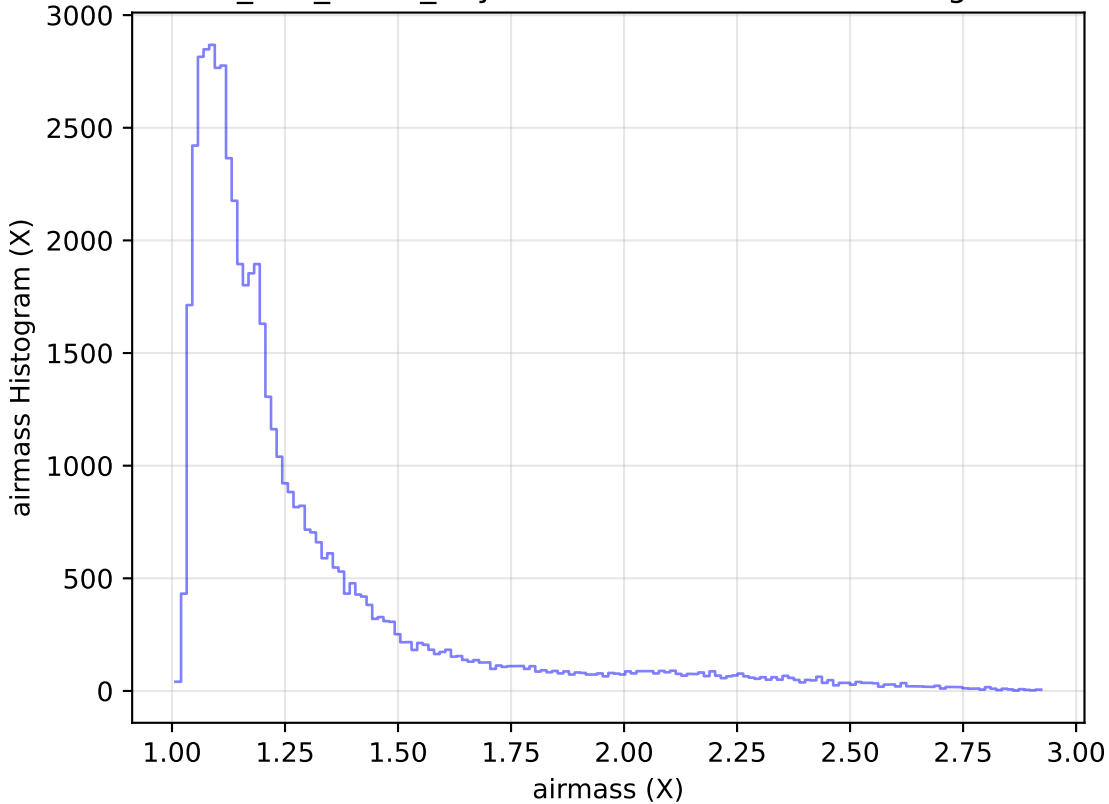
too_100_1v3.4_10yrs Yr 1 i band: airmass Histogram
