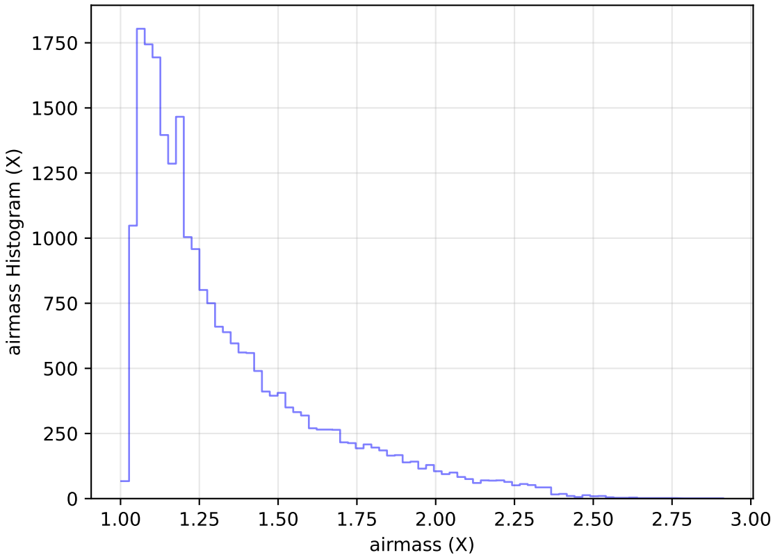
too_100_1v3.4_10yrs Yr 1 g band: airmass Histogram
