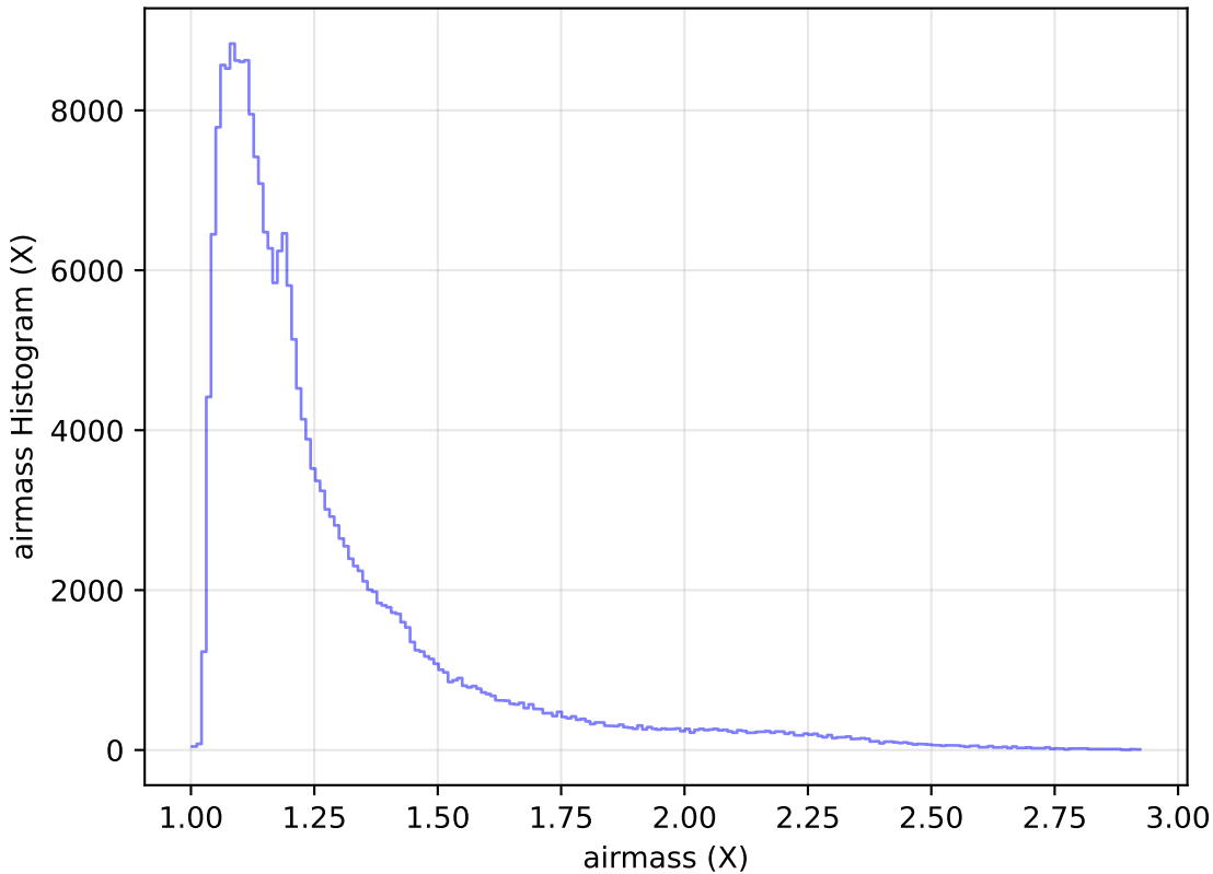
too_100_1v3.4_10yrs Yr 1 all bands: airmass Histogram
