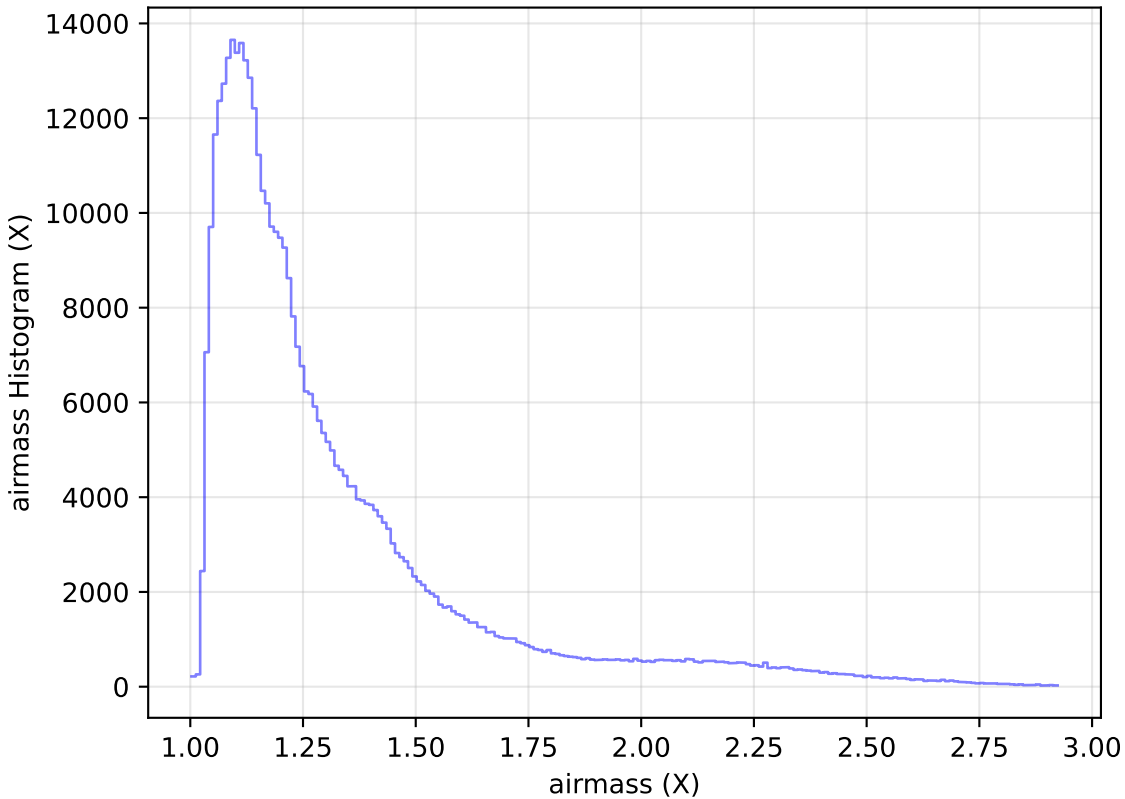
too_100_1v3.4_10yrs WFD z band: airmass Histogram
