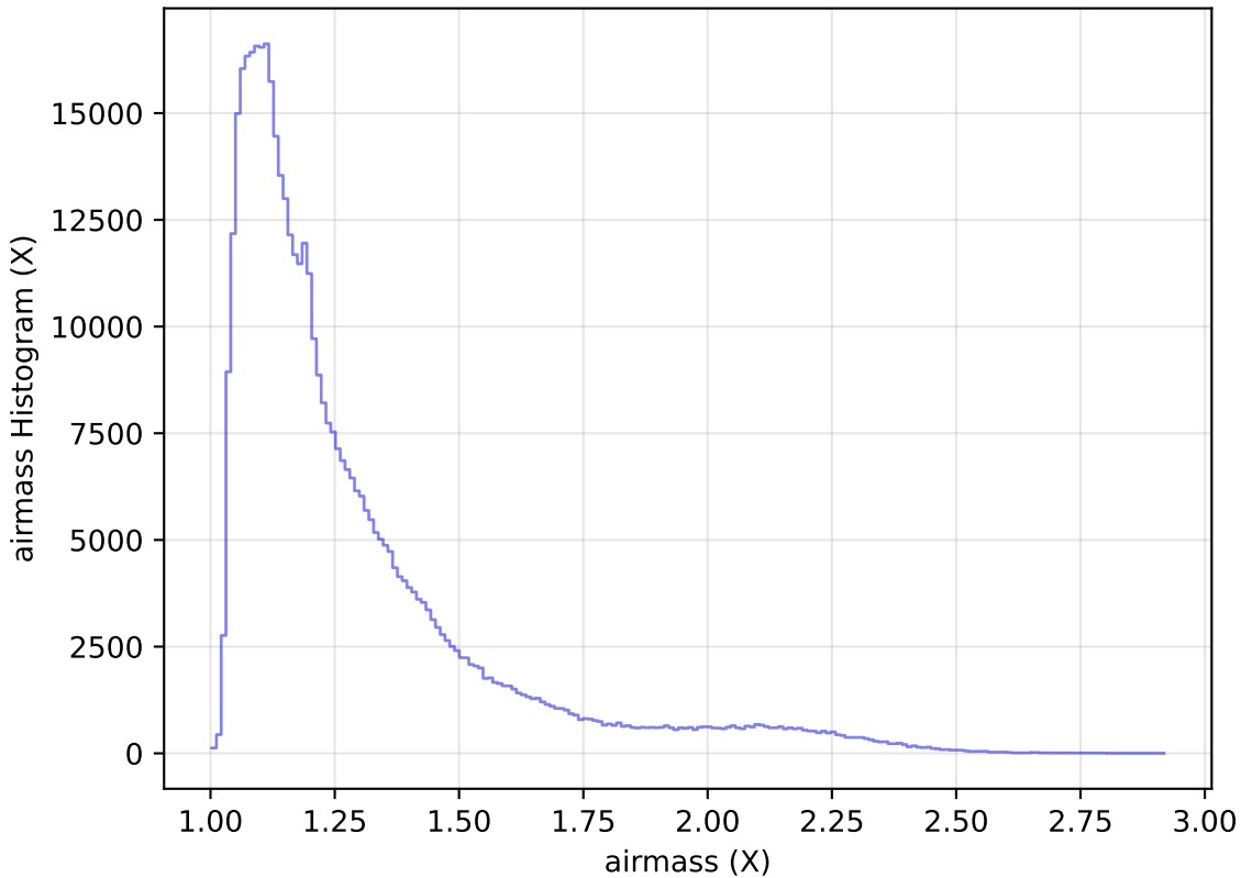
too_100_1v3.4_10yrs WFD r band: airmass Histogram
