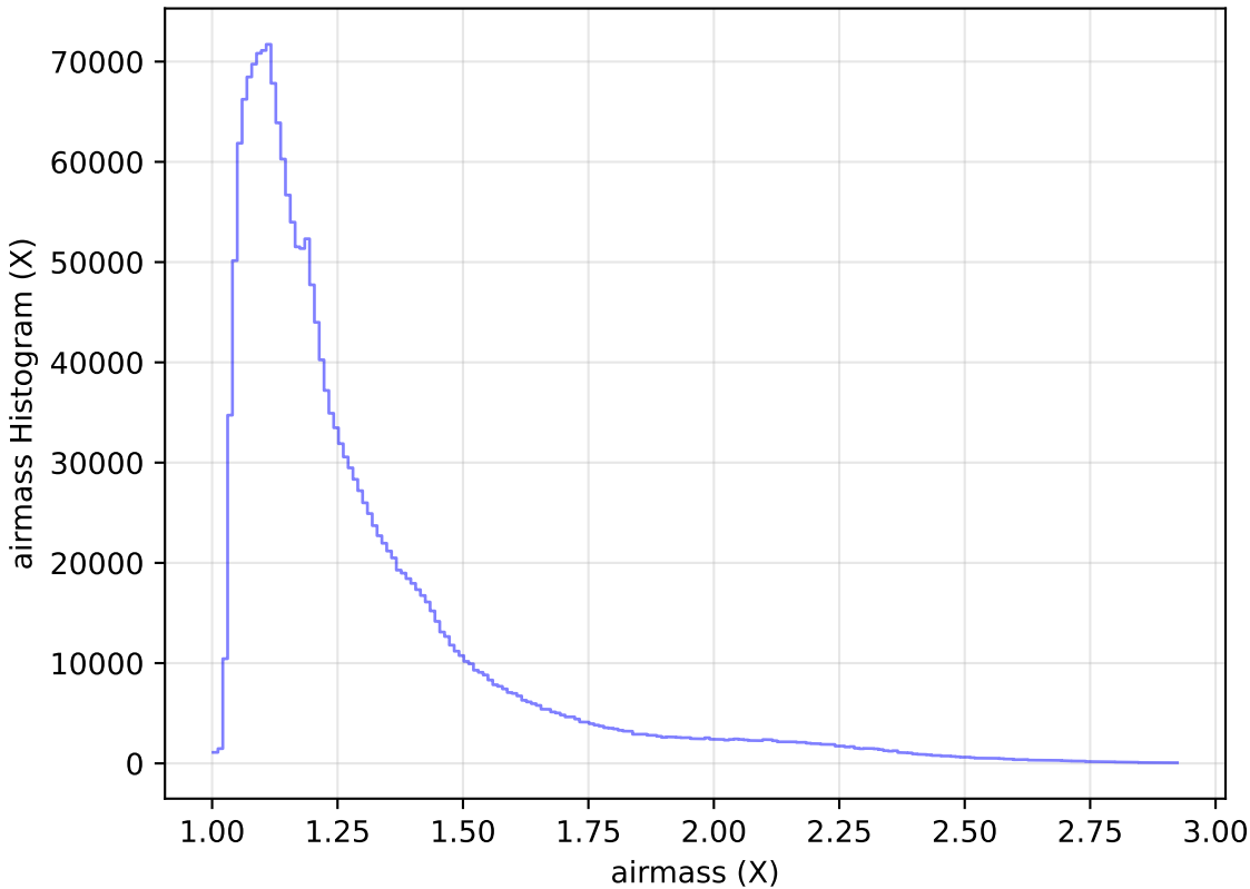
too_100_1v3.4_10yrs WFD all bands: airmass Histogram
