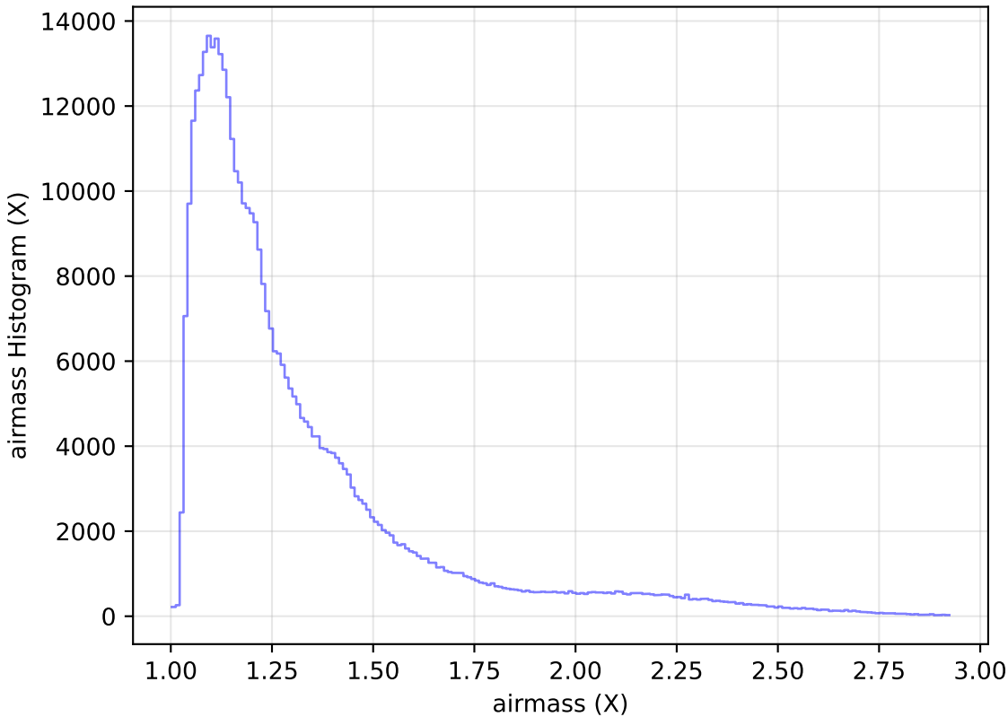
too_100_1v3.4_10yrs All sky z band: airmass Histogram
