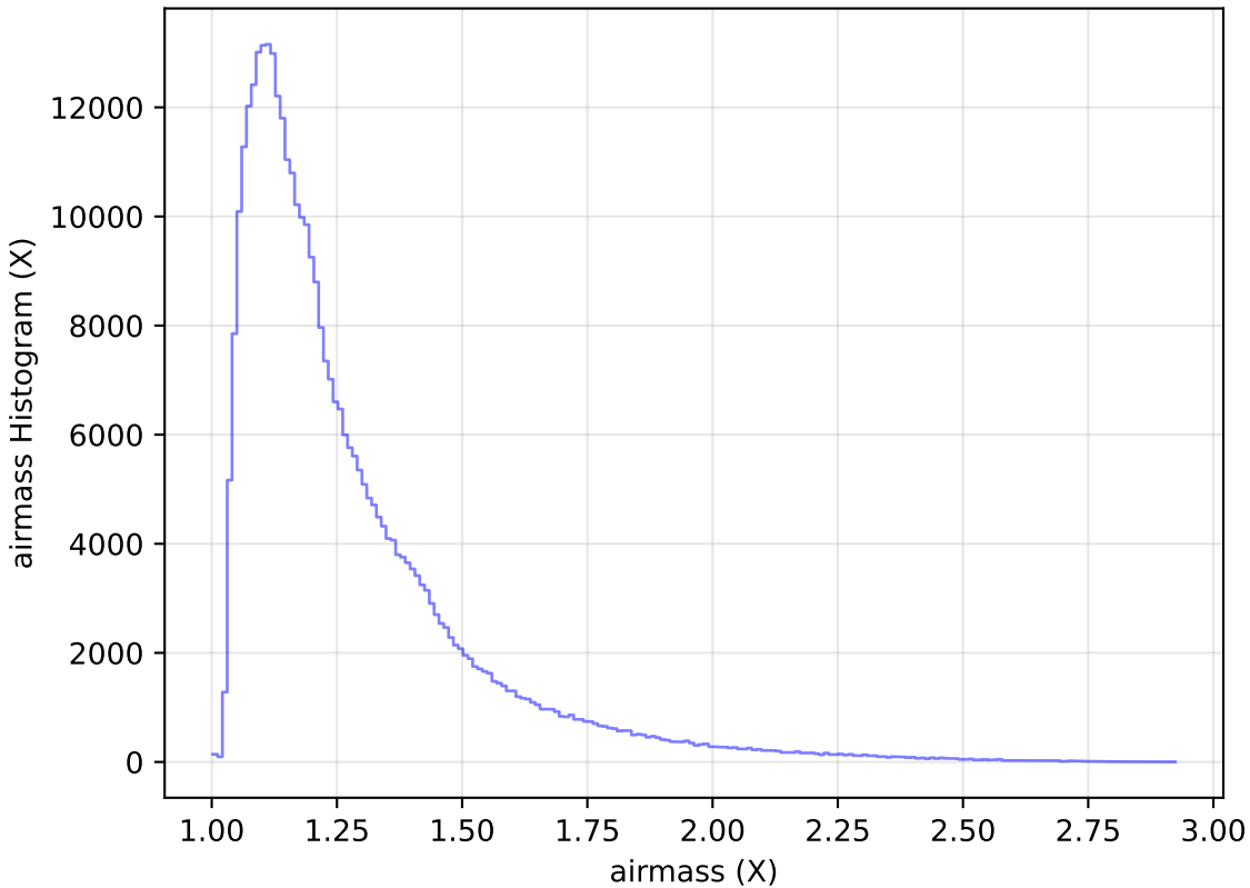
too_100_1v3.4_10yrs All sky y band: airmass Histogram
