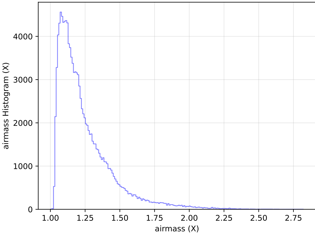
too_100_1v3.4_10yrs All sky u band: airmass Histogram
