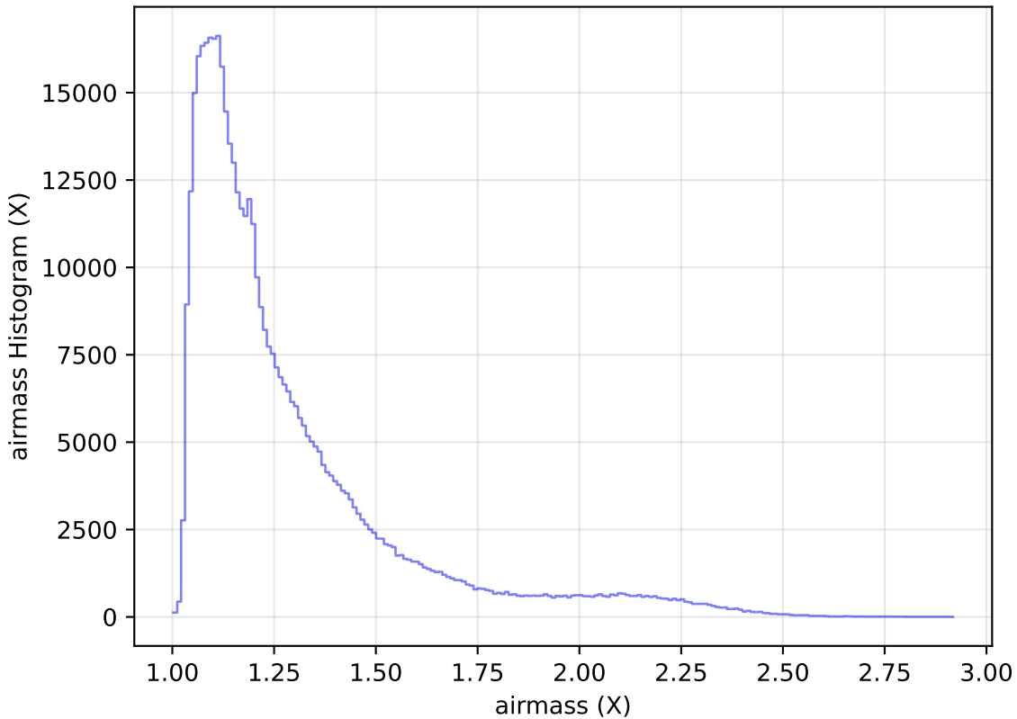
too_100_1v3.4_10yrs All sky r band: airmass Histogram
