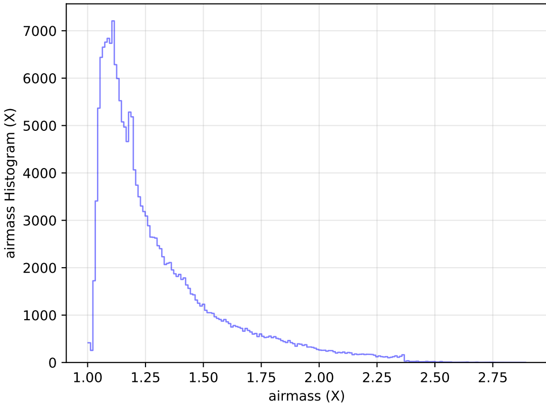
too_100_1v3.4_10yrs All sky g band: airmass Histogram
