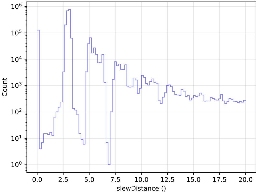
too_100_1v3.4_10yrs All visits: Zoom Slew Distance Histogram
