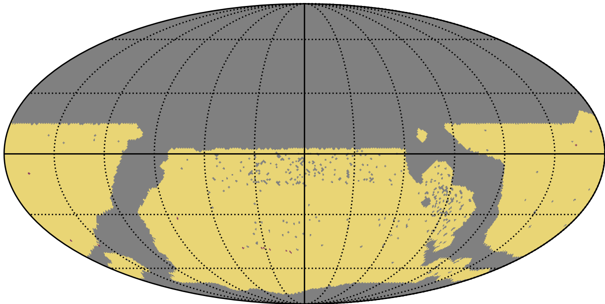
too_100_1v3.4_10yrs WFD: RapidRevisits
