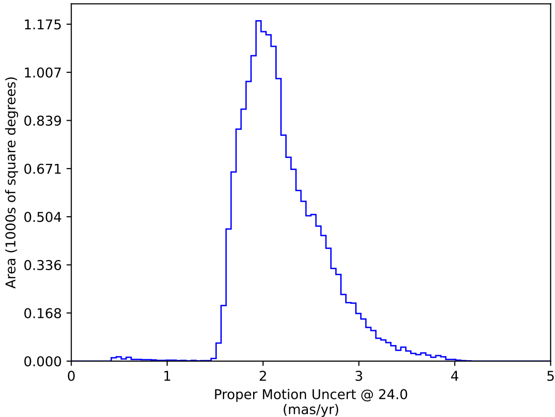
too_100_1v3.4_10yrs WFD: Proper Motion Uncert @ 24.0
