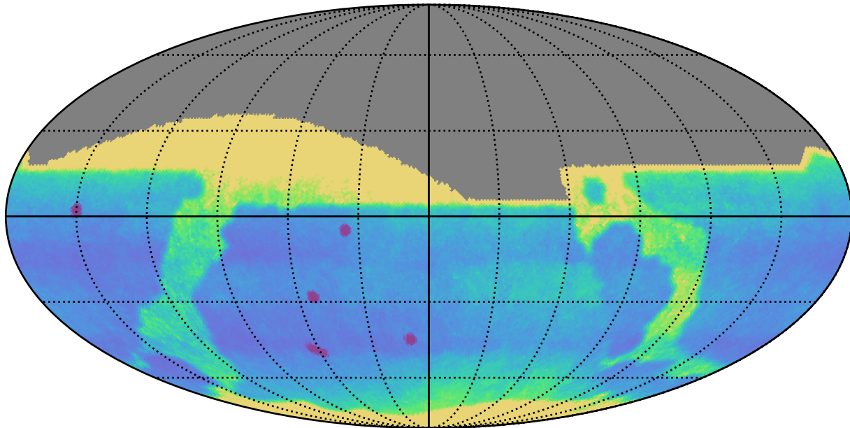
too_100_1v3.4_10yrs All sky: Proper Motion Uncert @ 24.0
