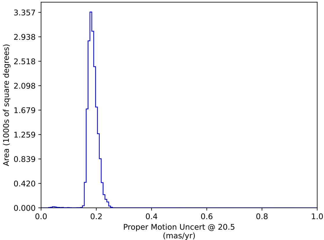
too_100_1v3.4_10yrs WFD: Proper Motion Uncert @ 20.5
