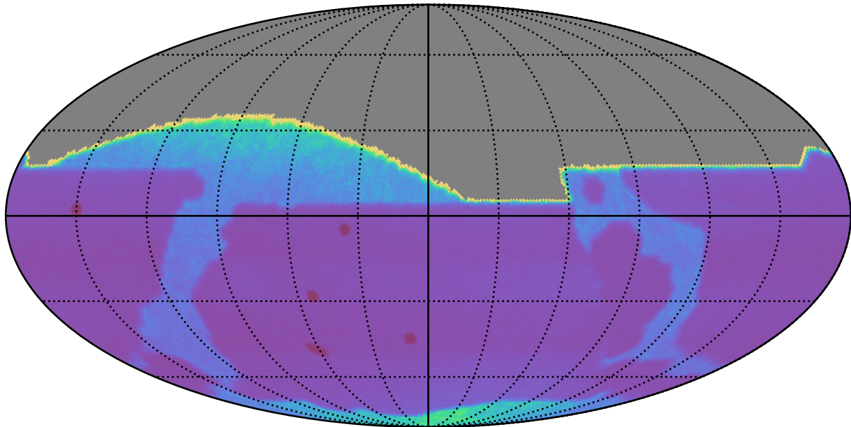
too_100_1v3.4_10yrs All sky: Proper Motion Uncert @ 20.5
