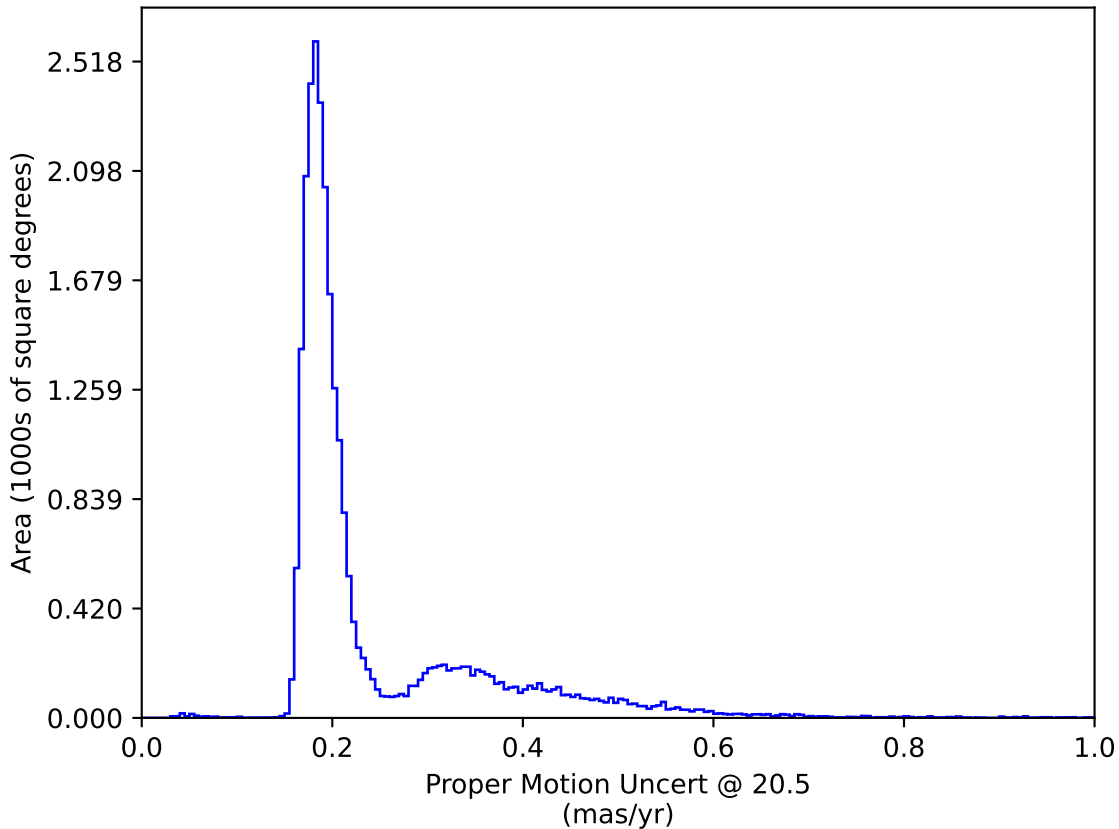
too_100_1v3.4_10yrs All sky: Proper Motion Uncert @ 20.5
