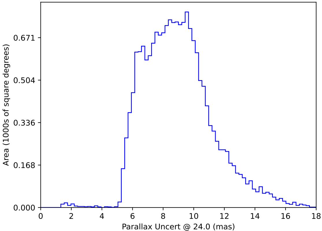
too_100_1v3.4_10yrs WFD: Parallax Uncert @ 24.0
