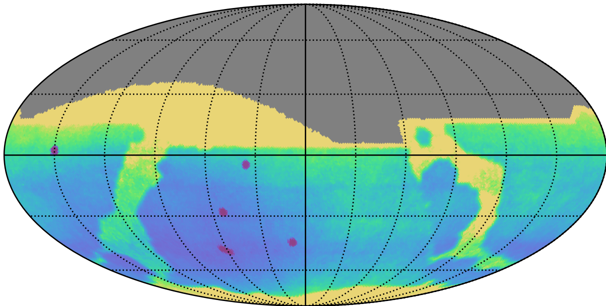
too_100_1v3.4_10yrs All sky: Parallax Uncert @ 24.0
