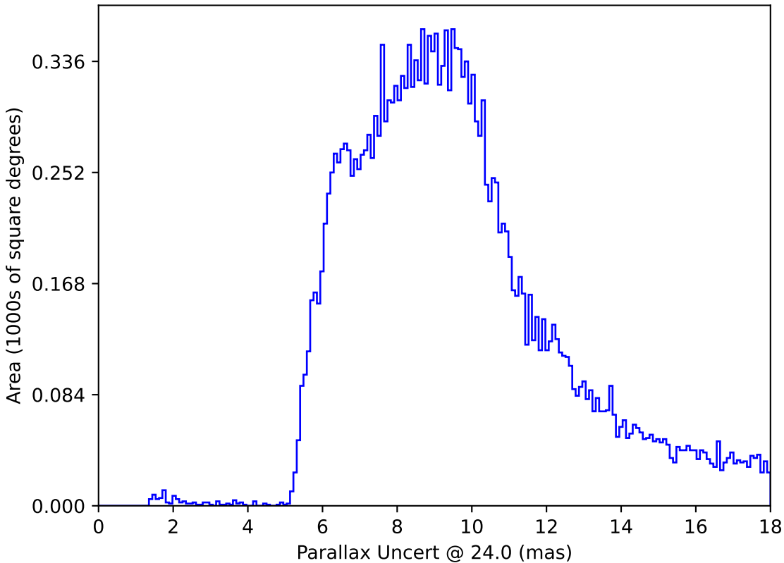
too_100_1v3.4_10yrs All sky: Parallax Uncert @ 24.0
