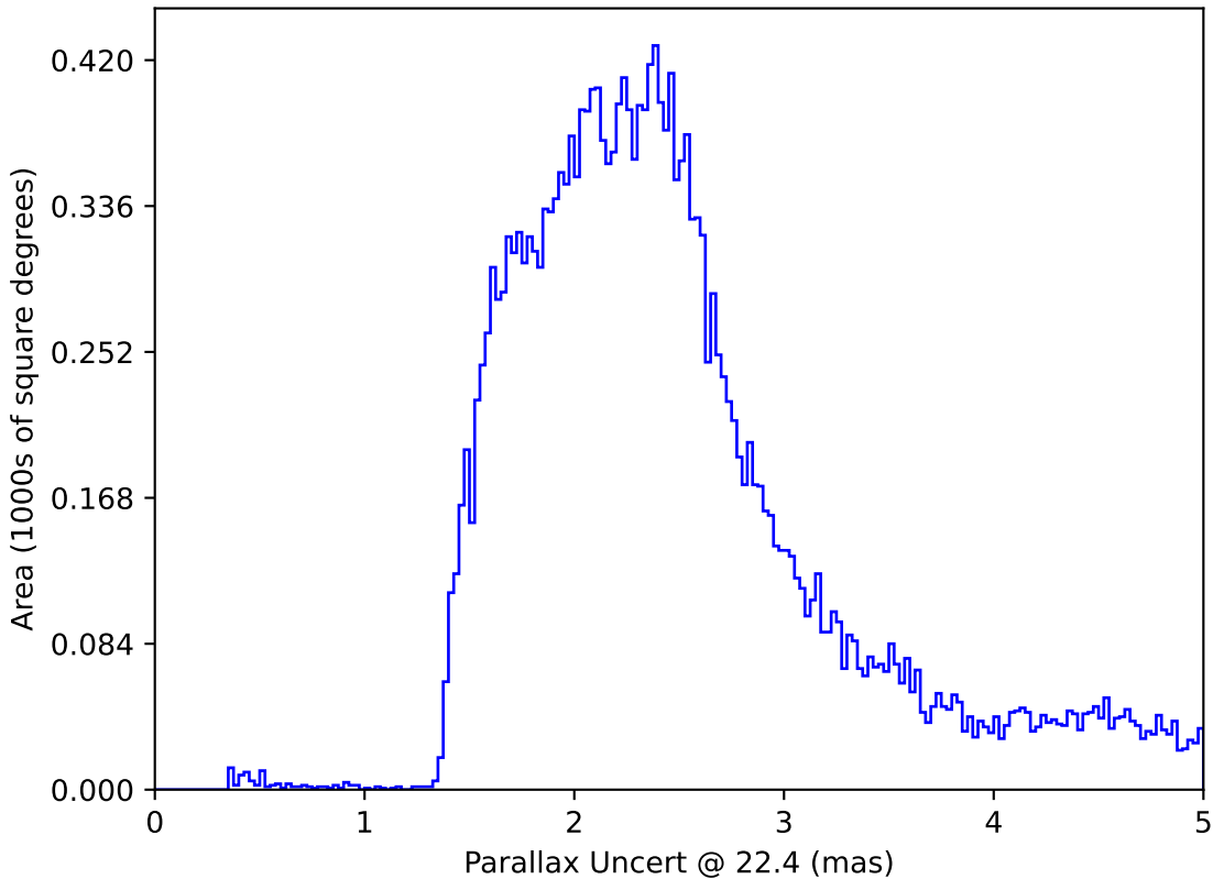
too_100_1v3.4_10yrs All sky: Parallax Uncert @ 22.4
