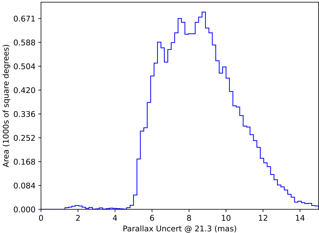
too_100_1v3.4_10yrs WFD y band only: Parallax Uncert @ 21.3
