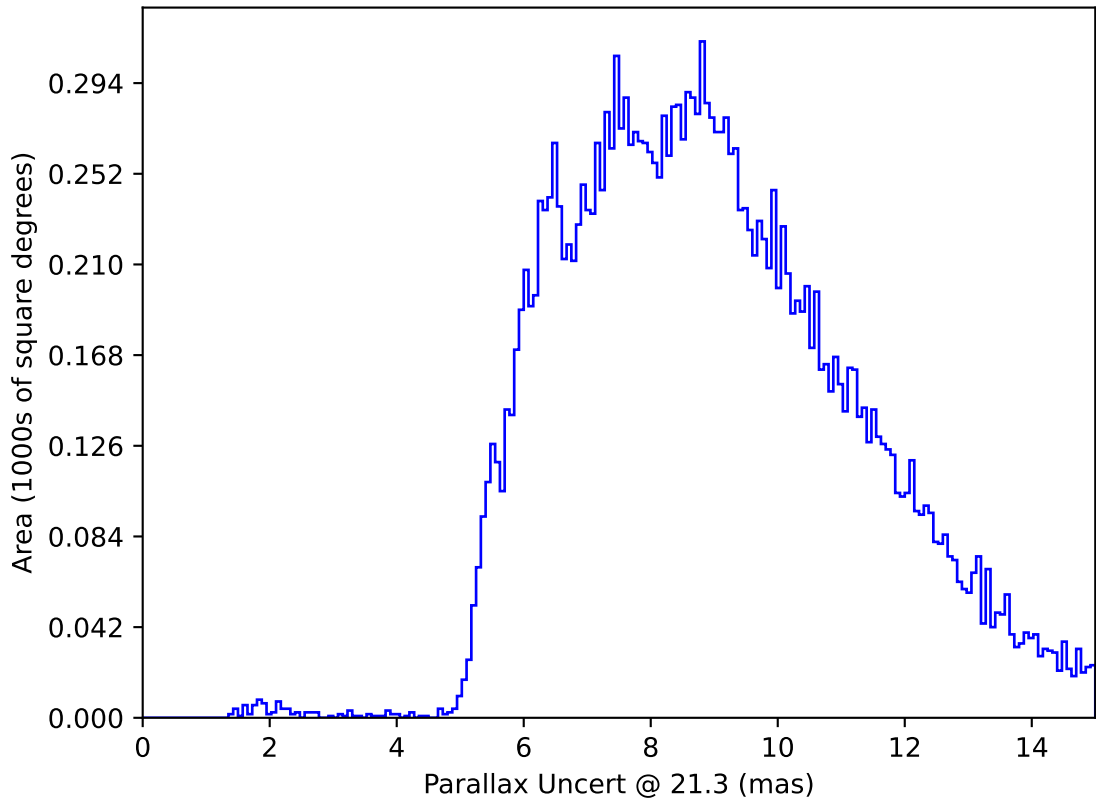
too_100_1v3.4_10yrs All sky y band only: Parallax Uncert @ 21.3
