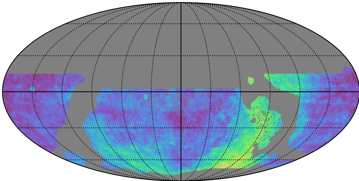
too_100_1v3.4_10yrs WFD: Parallax Coverage @ 24.0
