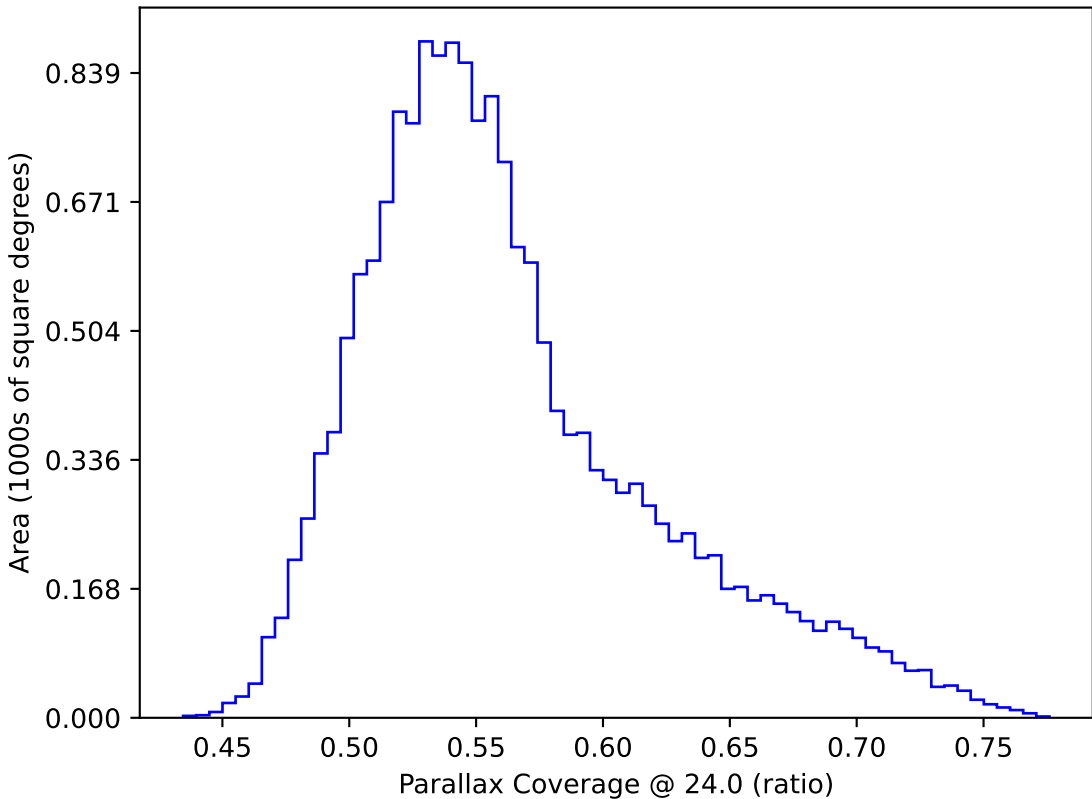
too_100_1v3.4_10yrs WFD: Parallax Coverage @ 24.0
