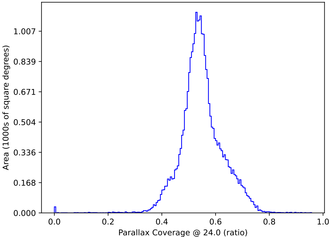
too_100_1v3.4_10yrs All sky: Parallax Coverage @ 24.0
