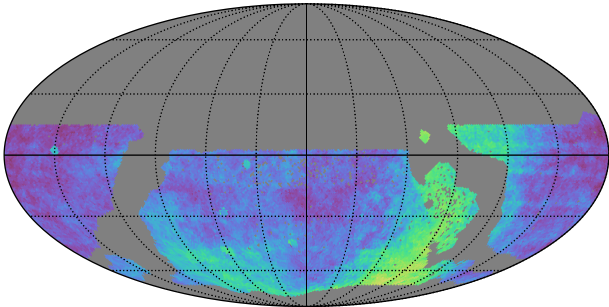
too_100_1v3.4_10yrs WFD: Parallax Coverage @ 22.4
