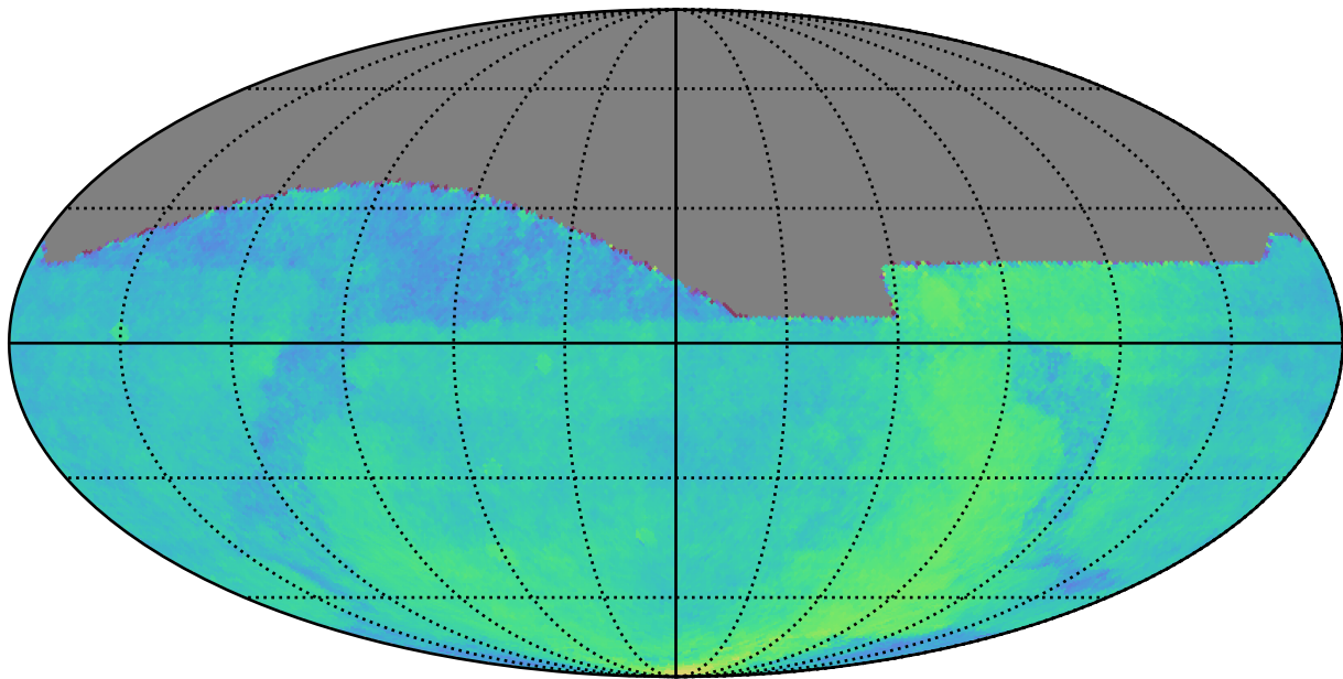
too_100_1v3.4_10yrs All sky: Parallax Coverage @ 22.4
