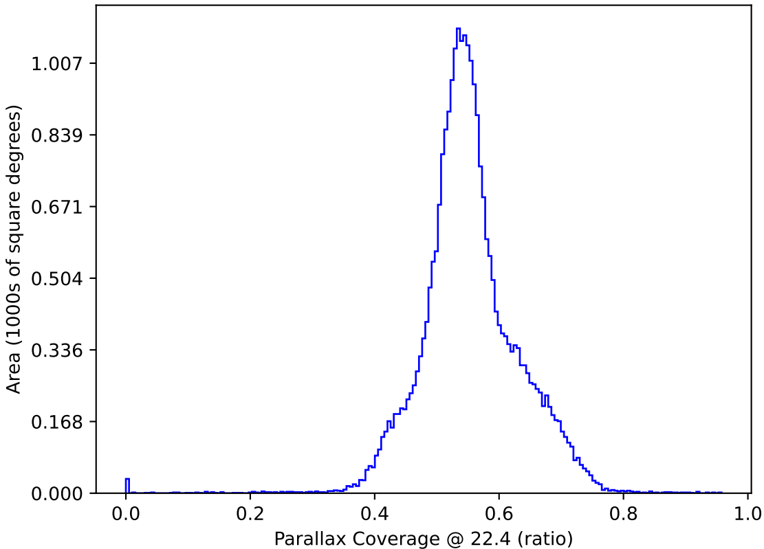
too_100_1v3.4_10yrs All sky: Parallax Coverage @ 22.4
