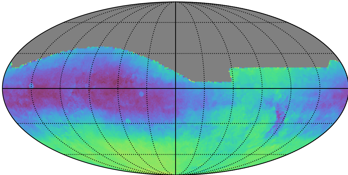
too_100_1v3.4_10yrs All sky: Parallax-DCR degeneracy @ 24.0
