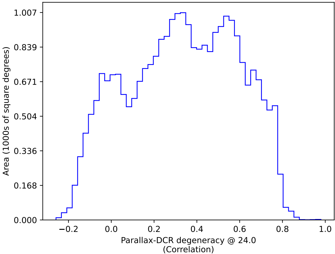
too_100_1v3.4_10yrs All sky: Parallax-DCR degeneracy @ 24.0
