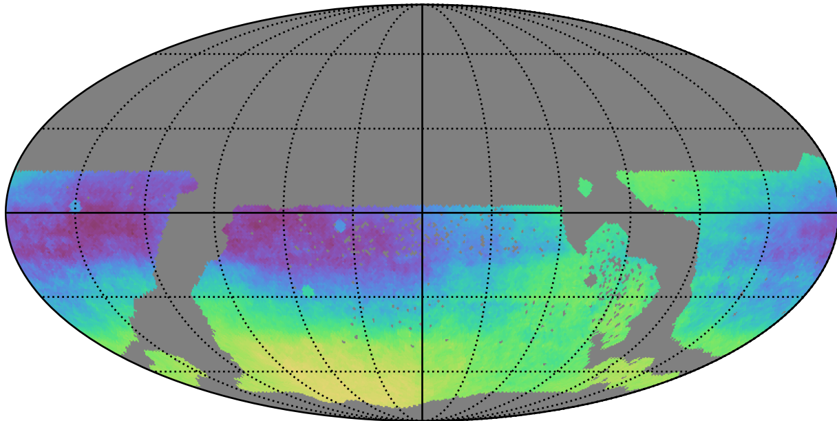
too_100_1v3.4_10yrs WFD: Parallax-DCR degeneracy @ 22.4
