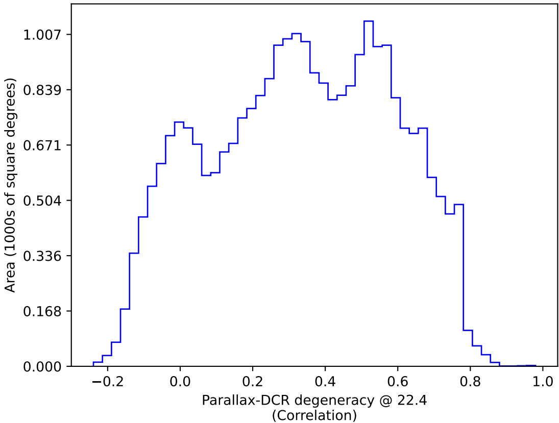
too_100_1v3.4_10yrs All sky: Parallax-DCR degeneracy @ 22.4
