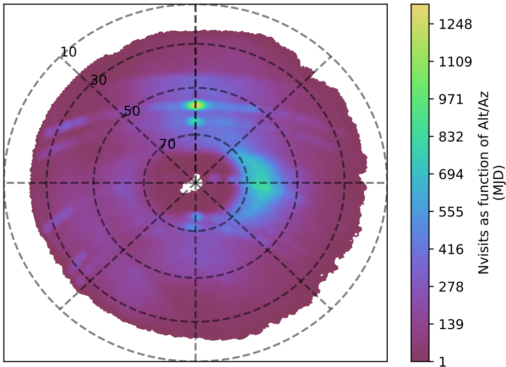
too_100_1v3.4_10yrs g band: Nvisits as function of Alt/Az
