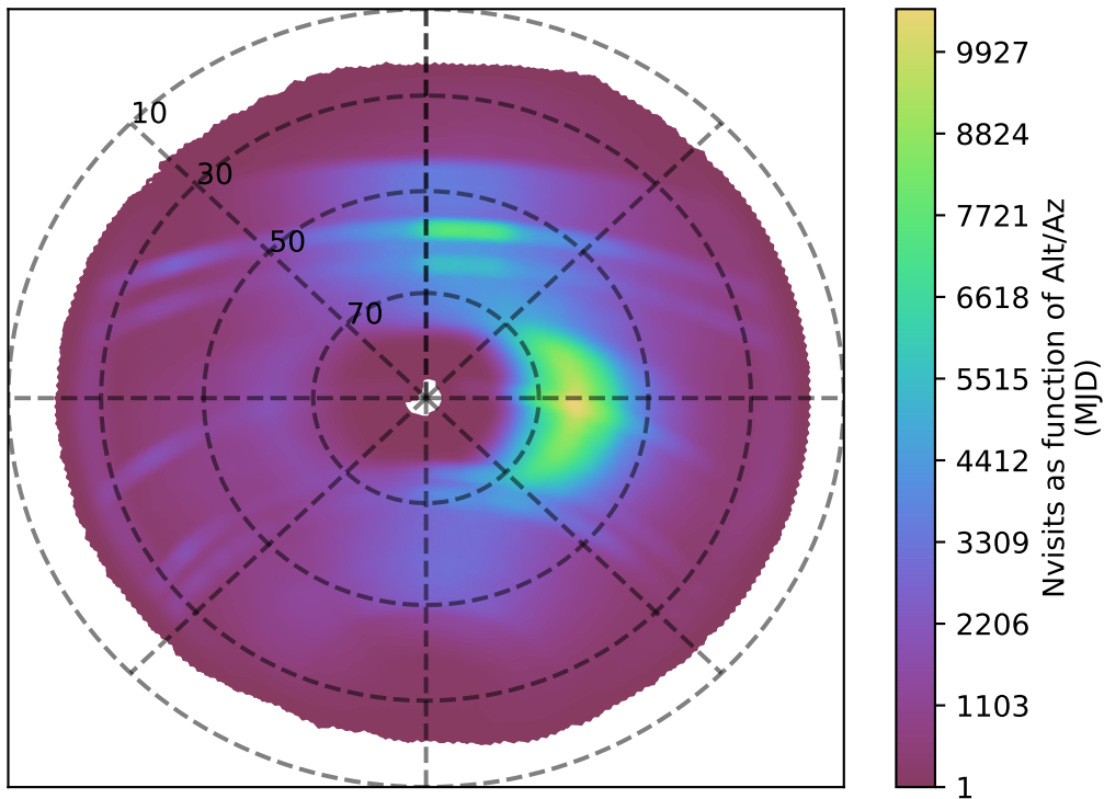
too_100_1v3.4_10yrs all bands: Nvisits as function of Alt/Az
