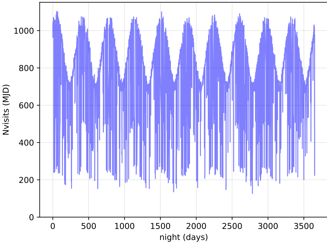
too_100_1v3.4_10yrs All visits: Nvisits
