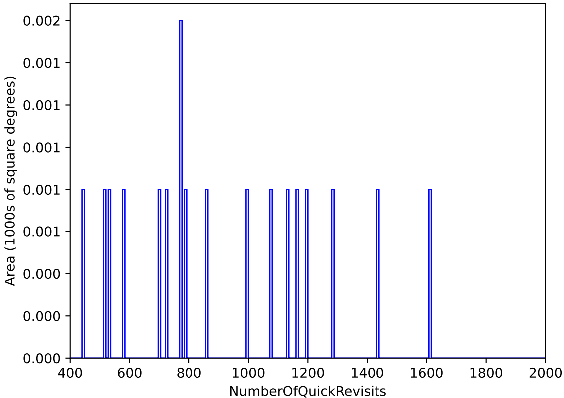
too_100_1v3.4_10yrs WFD: NumberOfQuickRevisits
