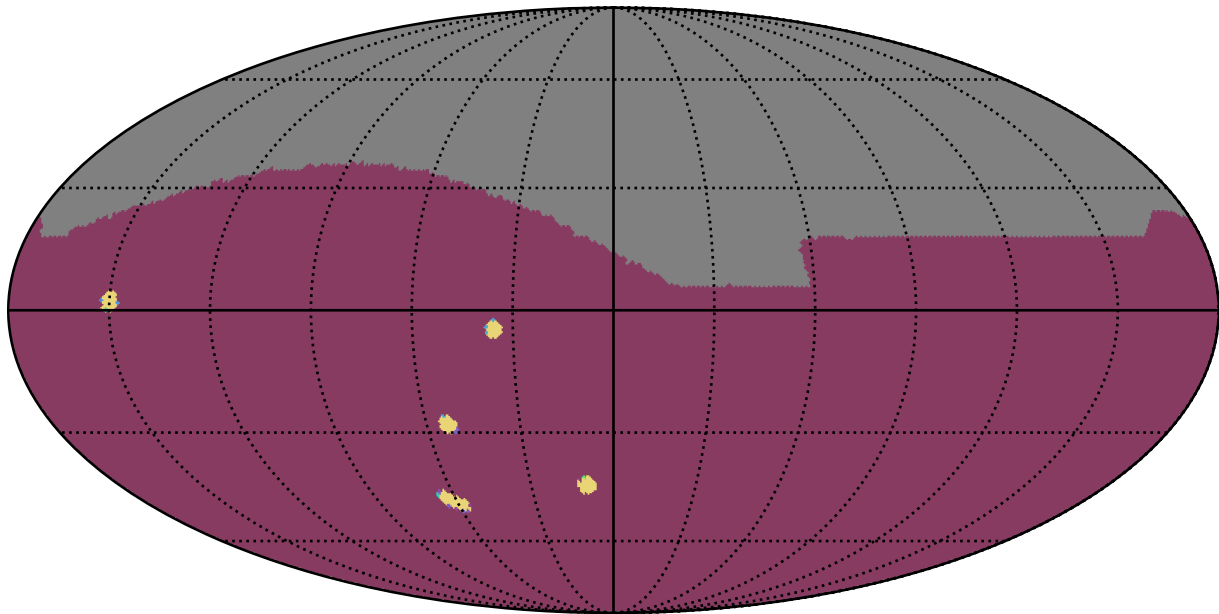
too_100_1v3.4_10yrs All sky: NumberOfQuickRevisits
