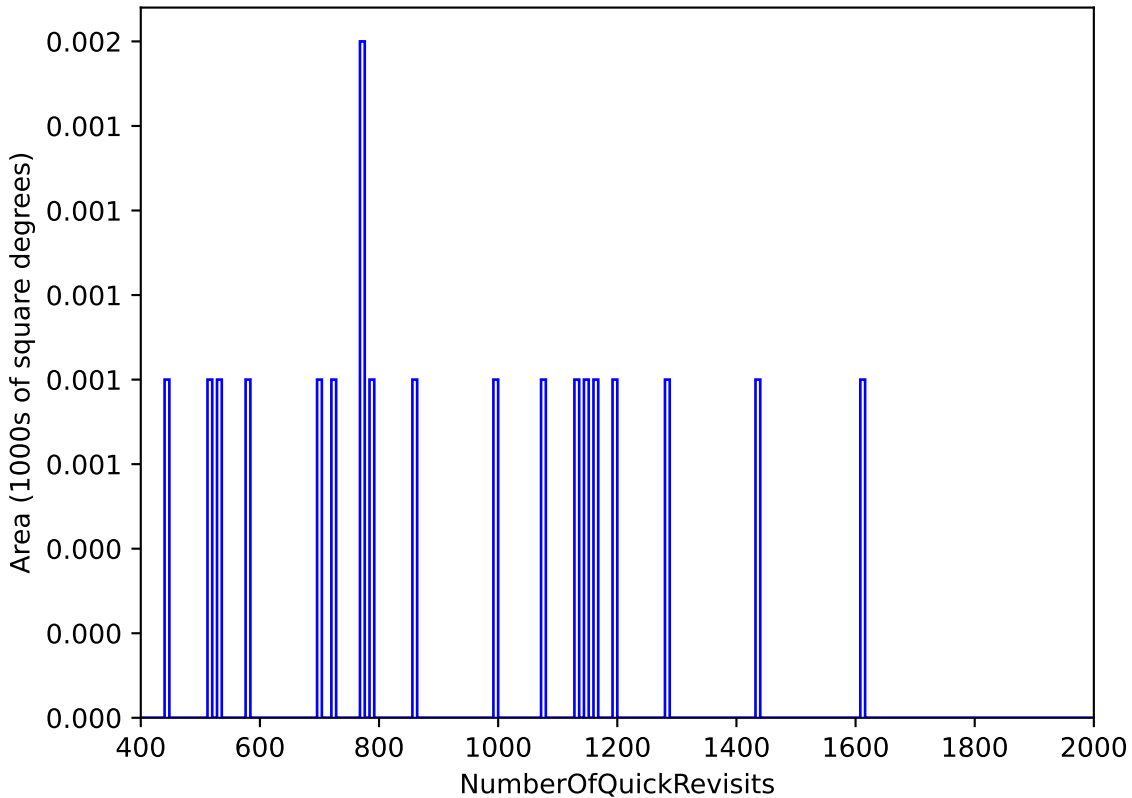
too_100_1v3.4_10yrs All sky: NumberOfQuickRevisits
