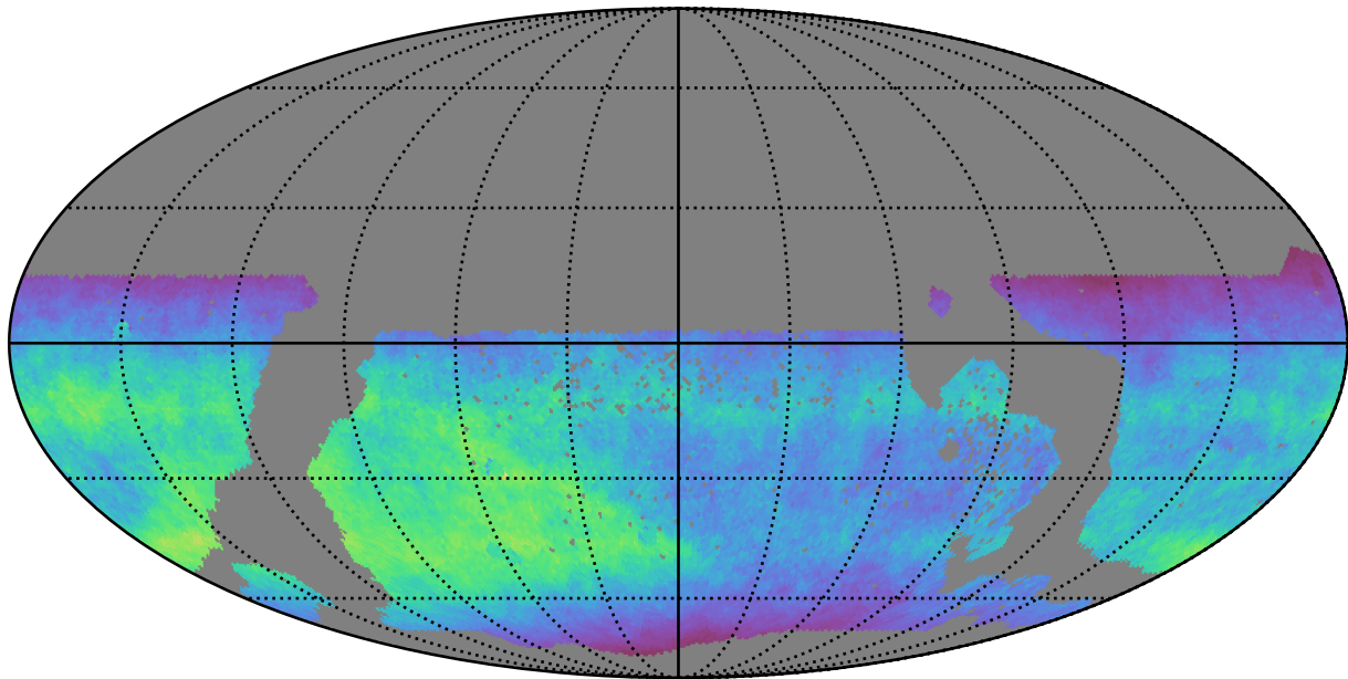
too_100_1v3.4_10yrs WFD z band: Normalized Teff
