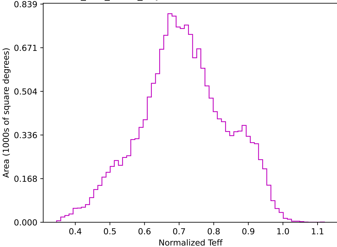
too_100_1v3.4_10yrs WFD z band: Normalized Teff
