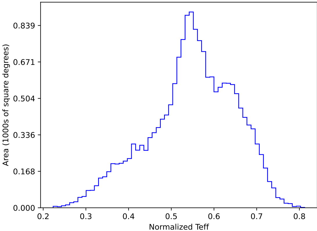
too_100_1v3.4_10yrs WFD y band: Normalized Teff
