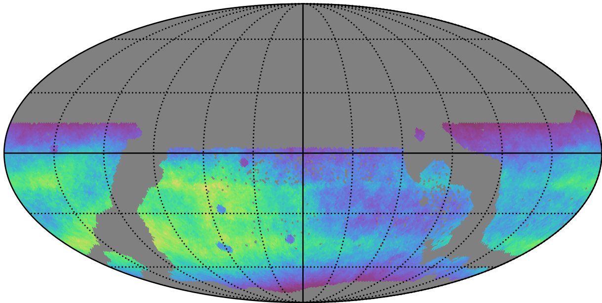
too_100_1v3.4_10yrs WFD r band: Normalized Teff
