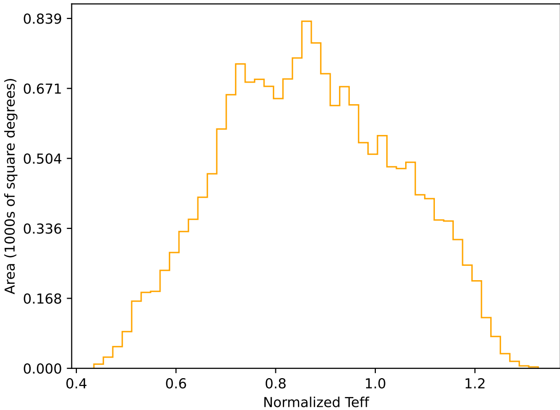
too_100_1v3.4_10yrs WFD r band: Normalized Teff
