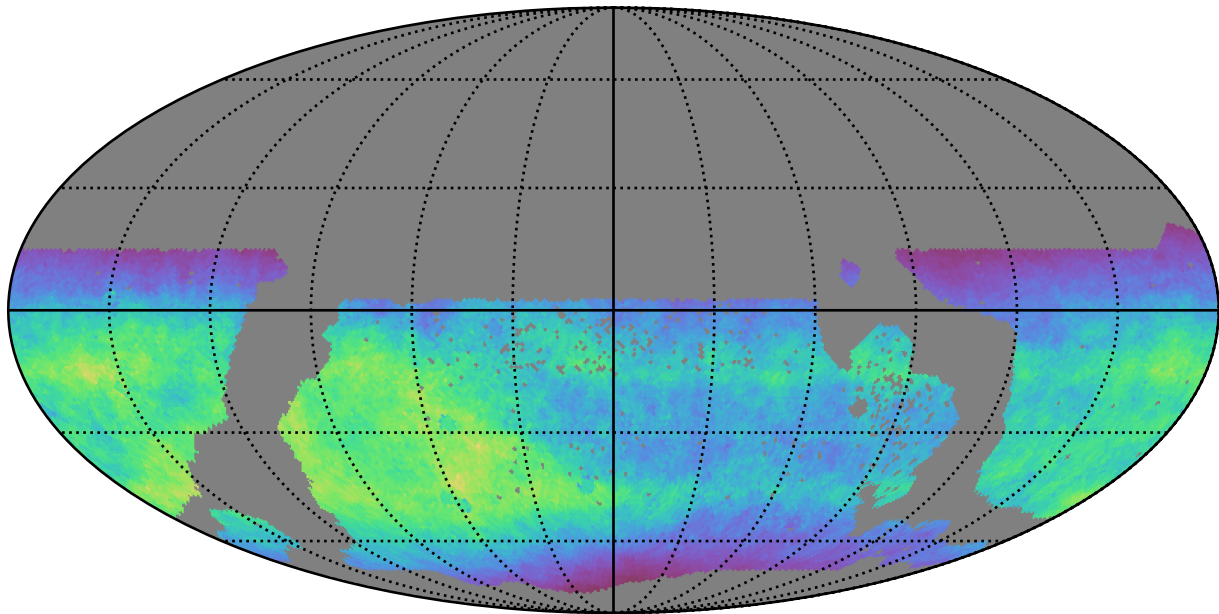
too_100_1v3.4_10yrs WFD i band: Normalized Teff
