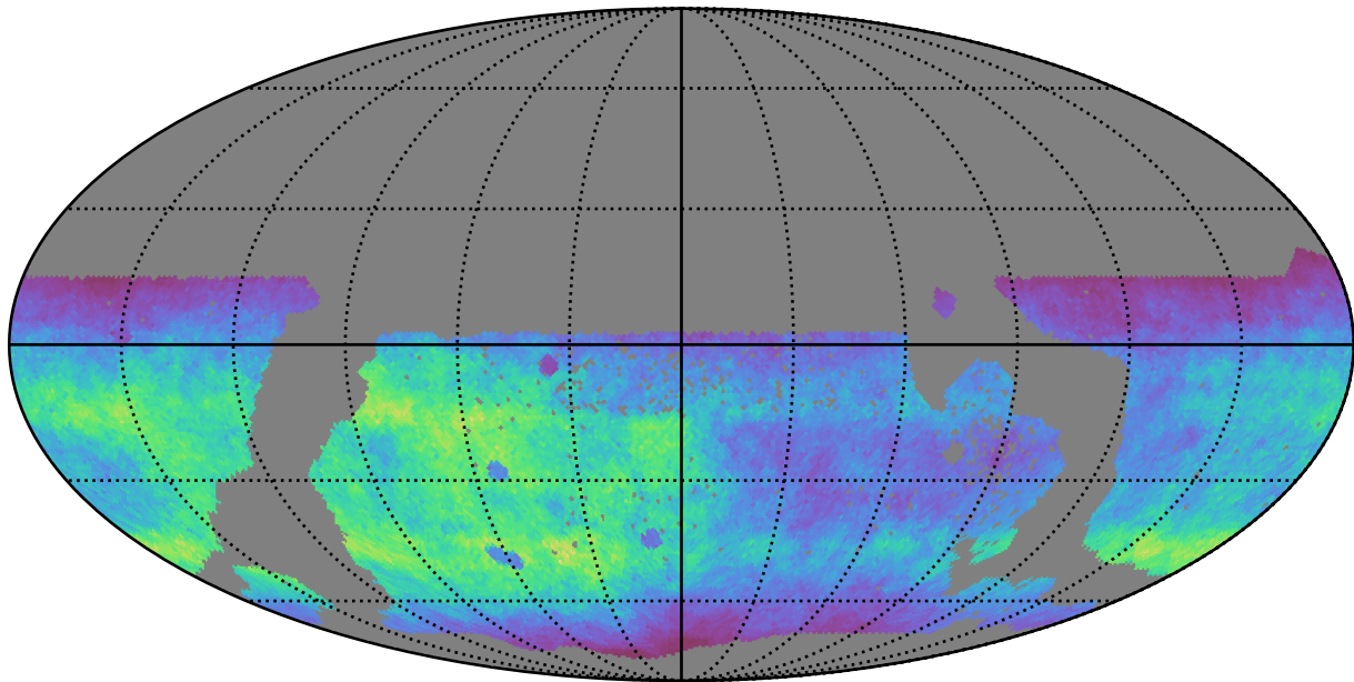
too_100_1v3.4_10yrs WFD g band: Normalized Teff
