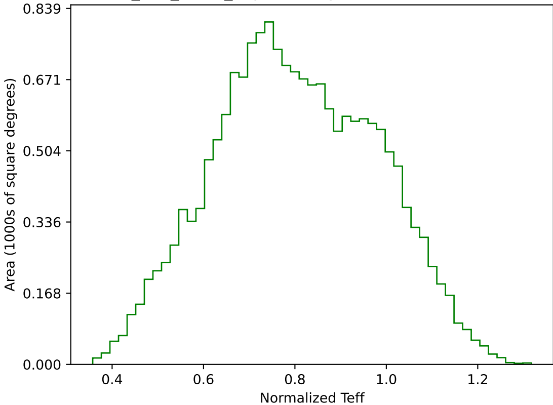
too_100_1v3.4_10yrs WFD g band: Normalized Teff
