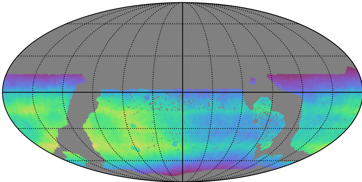
too_100_1v3.4_10yrs WFD all bands: Normalized Teff
